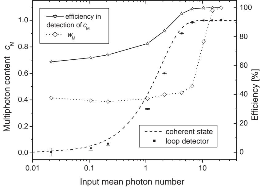
Fig. 5. Dependence of the measured multi-photon content c_M (black rectangles) on the mean photon number \mu of the input coherent state when detected with 15 channels of the device. The real (theoretical) multi-photon content c_M of the input state is shown by the dashed curve. Solid curve with stars (right axis) gives the ratio of the measured value of c_M to the real (theoretical) one. The dotted curve with hollow diamonds (right axis) gives the ratio w_M (for the definition, see text below).
